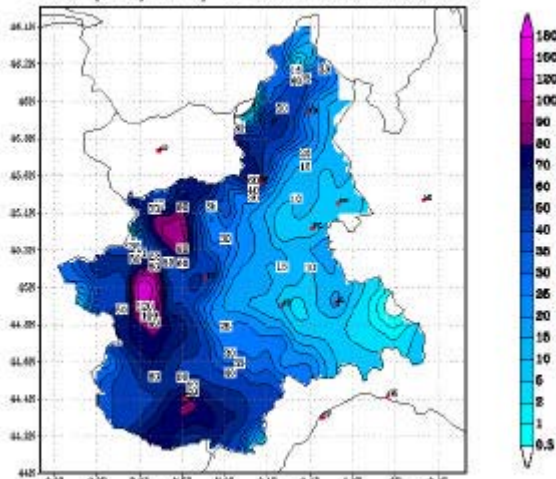
Prec. (mm/12hr) al 04MAY1999 12:00 UTC
