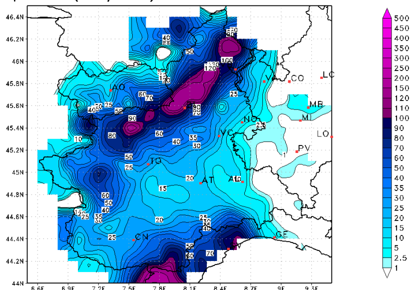
Precipitation (mm/24hr) at Thu 24NOV2016 00:00 UTC
