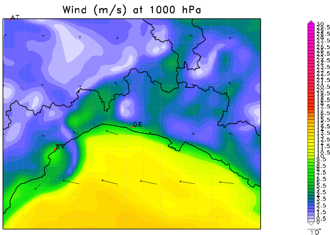
COSMO-I2 - LAMIN_ITALY_0025 - Wed 23 NOV 2016 12 UTC - Analysis
