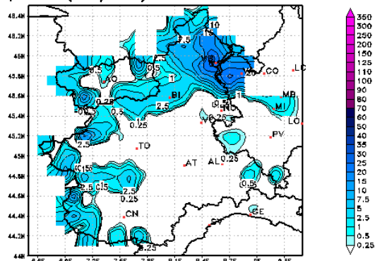
Precipitation (mm/06hr) at Fri 25NOV2016 18:00 UTC
