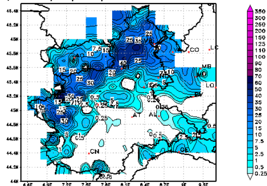
Precipitation (mm/06hr) at Fri 25NOV2016 12:00 UTC
