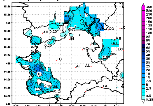
Precipitation (mm/06hr) at Sat 26NOV2016 00:00 UTC
