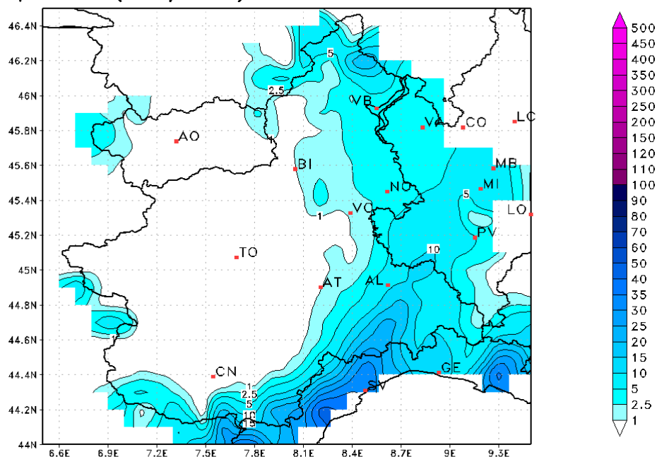
Precipitation (mm/24hr) at Mon 21NOV2016 00:00 UTC
